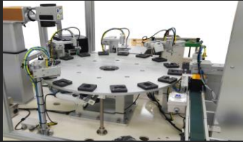
Product Name : MOB Marking
